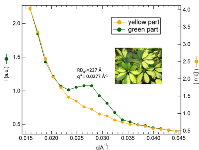
Fig. 2. SANS profiles of D_2O -infiltrated variegated Schefflera arboricola leaves recorded on the green and yellow parts of the leaf. The peak position and the calculated RD_{q^*} value are also indicated. The measurements were carried out at the BNC Yellow Submarine SANS instrument (SD = 5.5 m; collimation, 4 m; \lambda = 7.6 Å).
